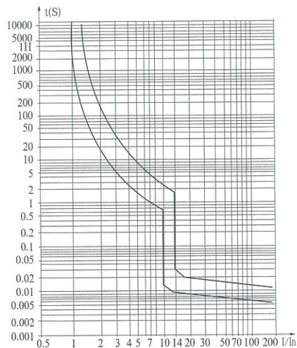
HB45-63-D型曲线(10 ~ 14In)
