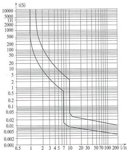
HM45-100H-C型曲线(7 ~ 10In)
