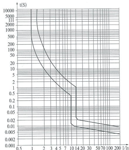
HM45-100-D型曲线(10 ~ 14In)
